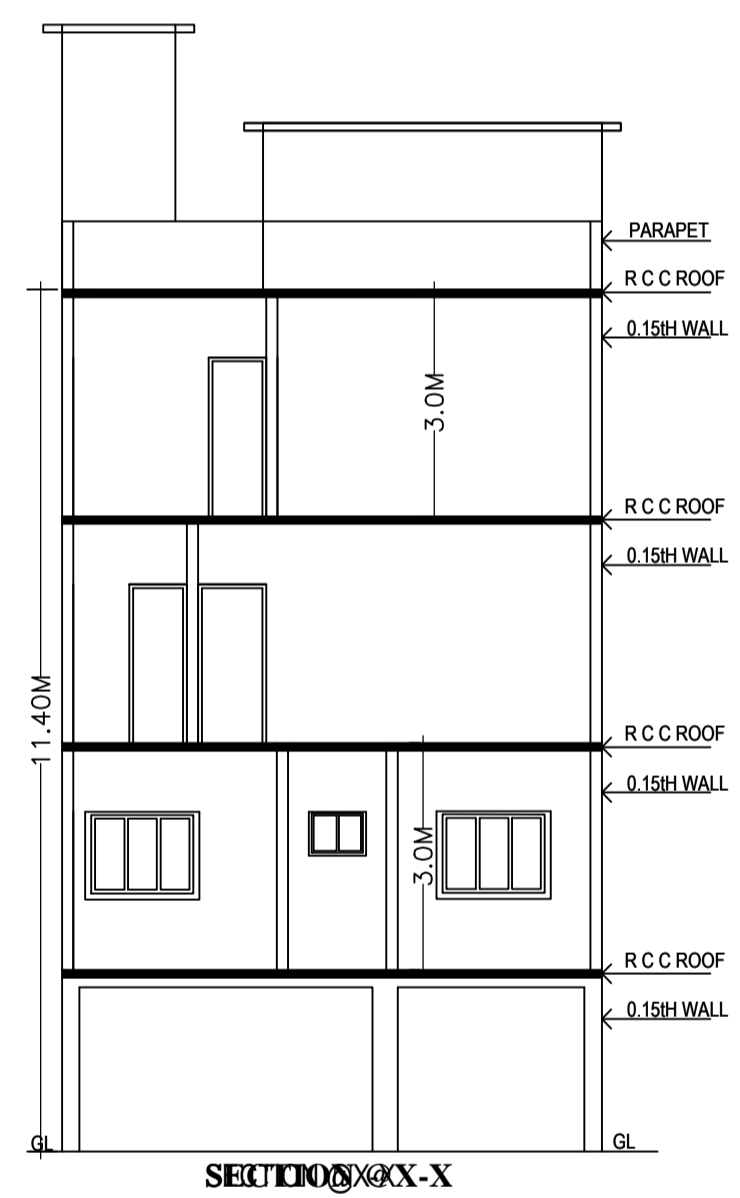
SECTION X-X
